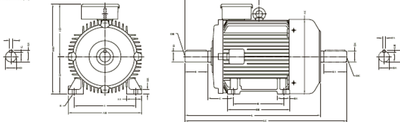
FOOT MOUNTING (B3)
