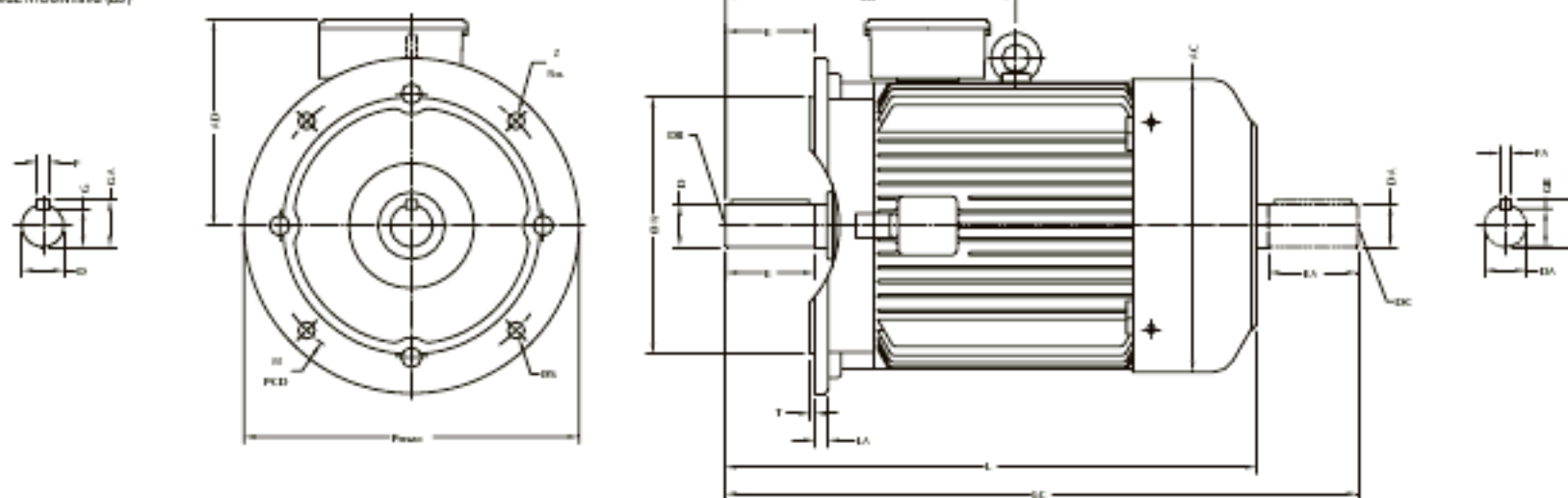
FLANGE MOUNTING (B5)
